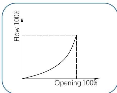
Opening-Flow Curve
